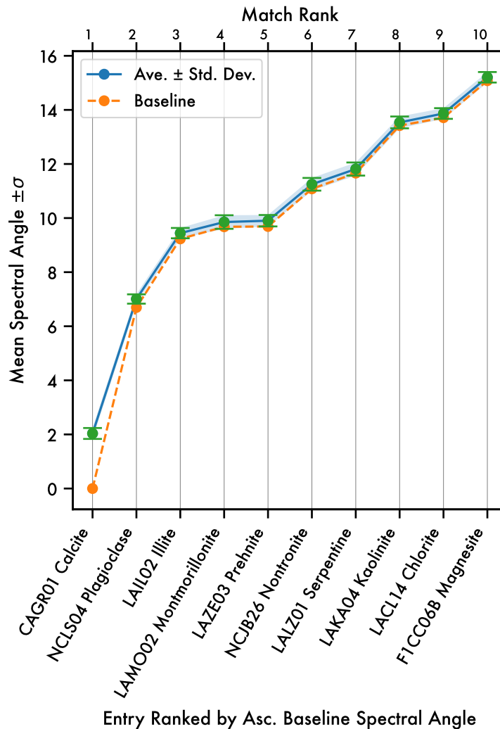
CAGR01 Calcite Mean Spectral Angle Match
